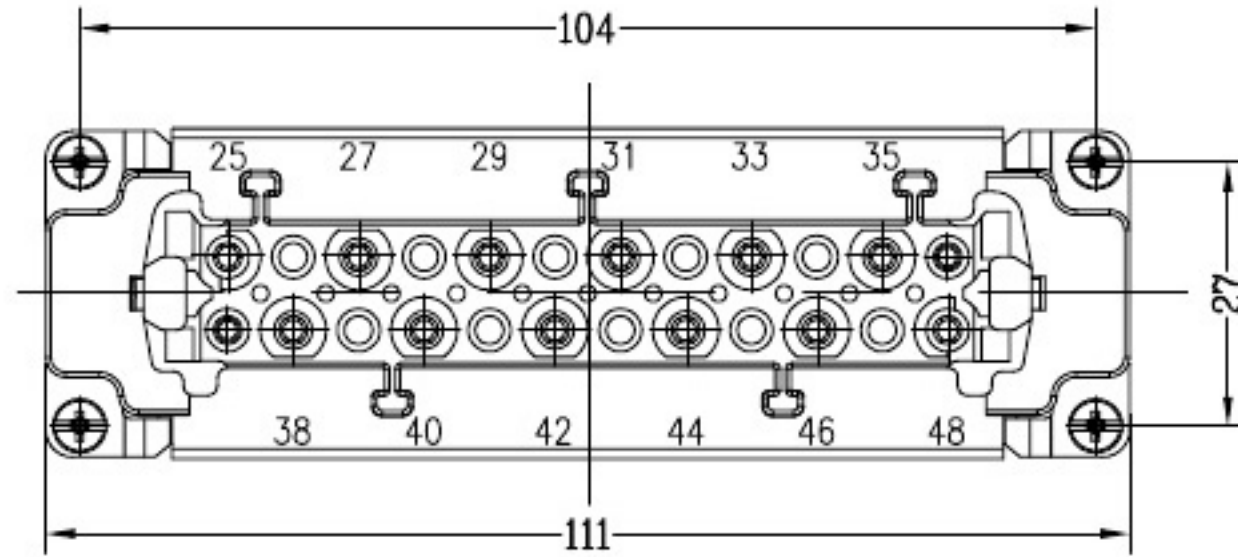
contact arrangement
