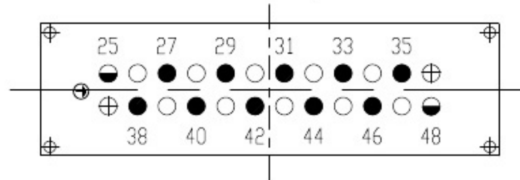
contact arrangement
