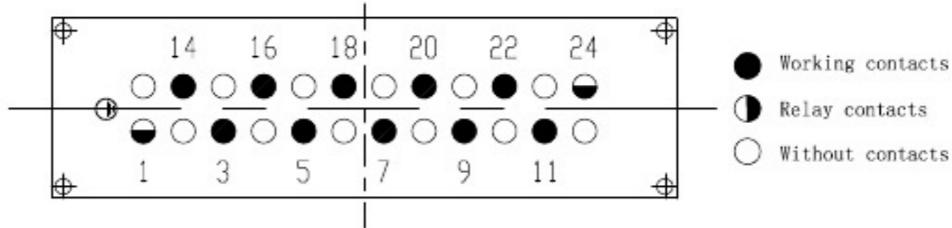
contact arrangement
