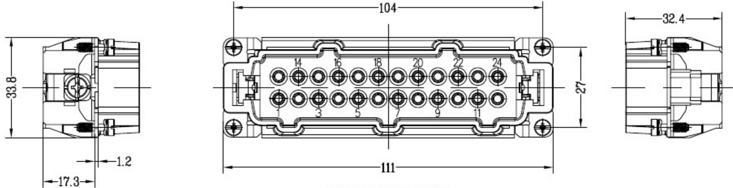
contact arrangement
