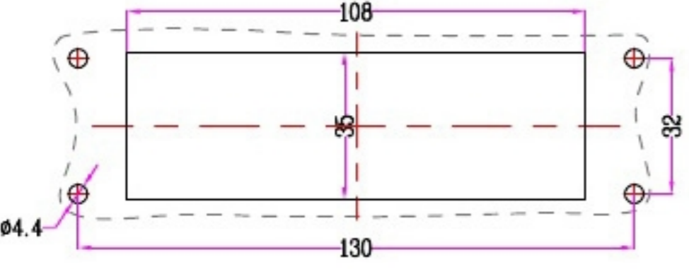
Bulkhead mounting Panel cut out
